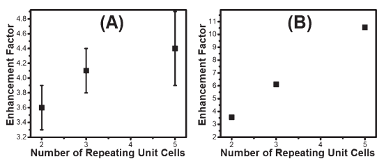
Figure 5. (A) Experimental enhancement of the quantum dot emission intensity because of the increased number of plasmon resonators as a function of the repeated number of unit cells, and (B) simulated enhancement factors derived from the calculated decay rates for two-, three-, and five-time repeating unit cell structures compared to a single unit cell structure using numerical simulations.
